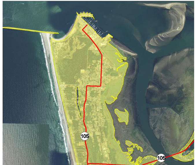
Figure 1. Aerial view of the community of West Port between South Bay (right) and the Pacific Ocean (left). The tsunami hazard zone is shaded in yellow. Highways are marked by solid red lines.
